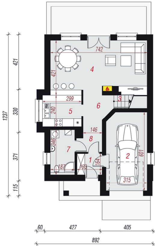
PARTER
