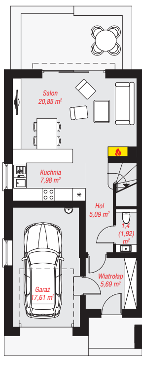
PARTER: 58,62 (59,14) m 2
