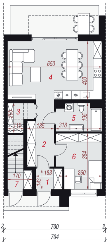
PARTER
