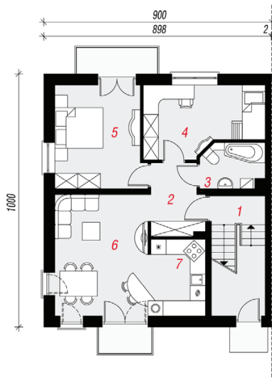
PARTER
