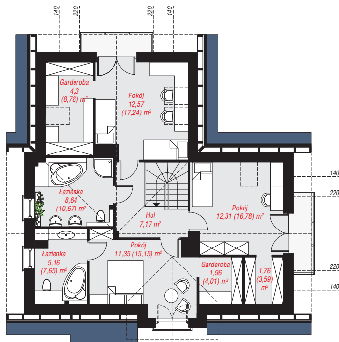
PODDASZE: 65,22 (91,04) m 2
